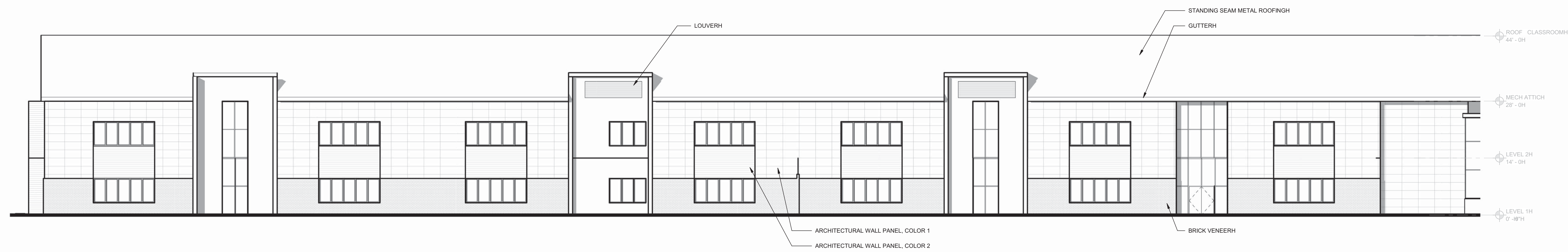
1H NORTH ELEVATION - SECTOR CH 3/32" = 1" = 8'H
