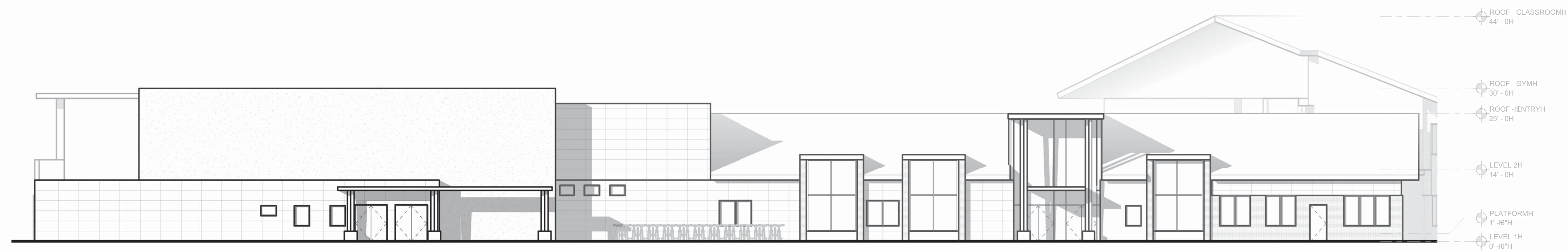
4H WEST ELEVATION 3/32" = 1'-0"
