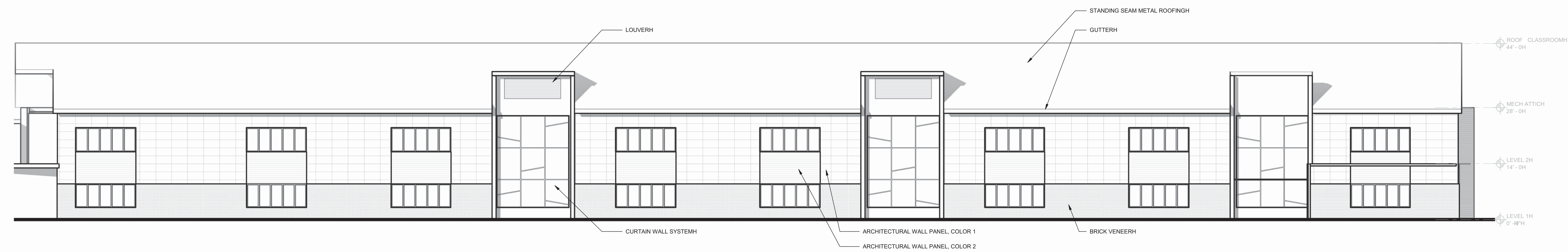
2H SOUTH ELEVATION - SECTOR CH 3/32" = 1" = 8'H
