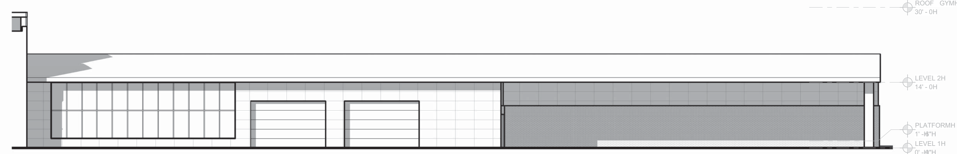
3H SOUTH ELEVATION - SECTOR AH 3/32" = 1'-0"
