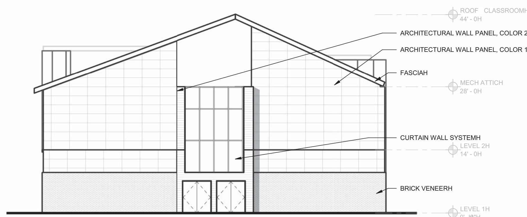
3H EAST ELEVATION - SECTOR CH 3/32" = 1" = 8'H
