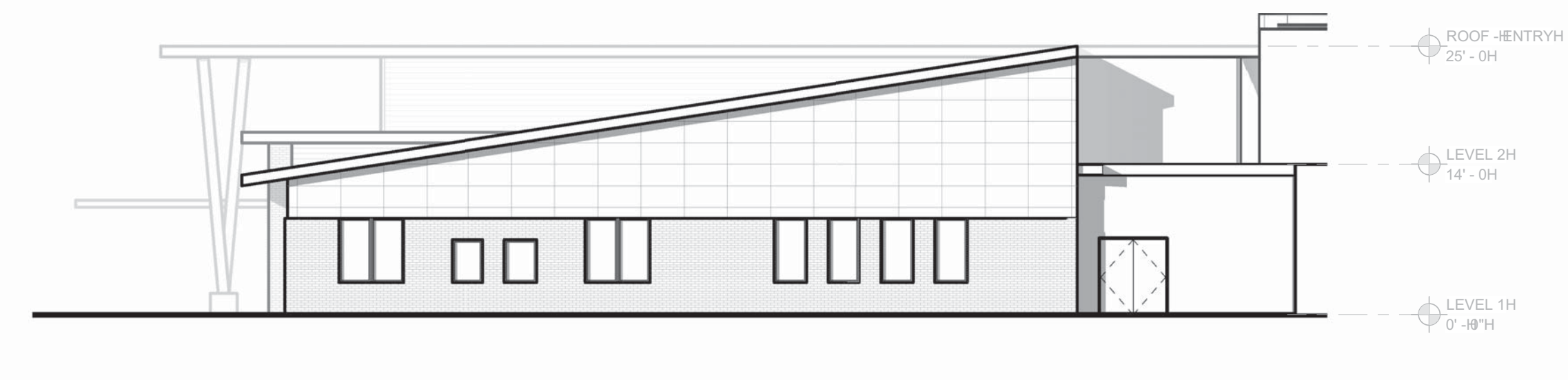
7H SOUTH ELEVATION - SECTOR BH 3/32" = 1'-0"
