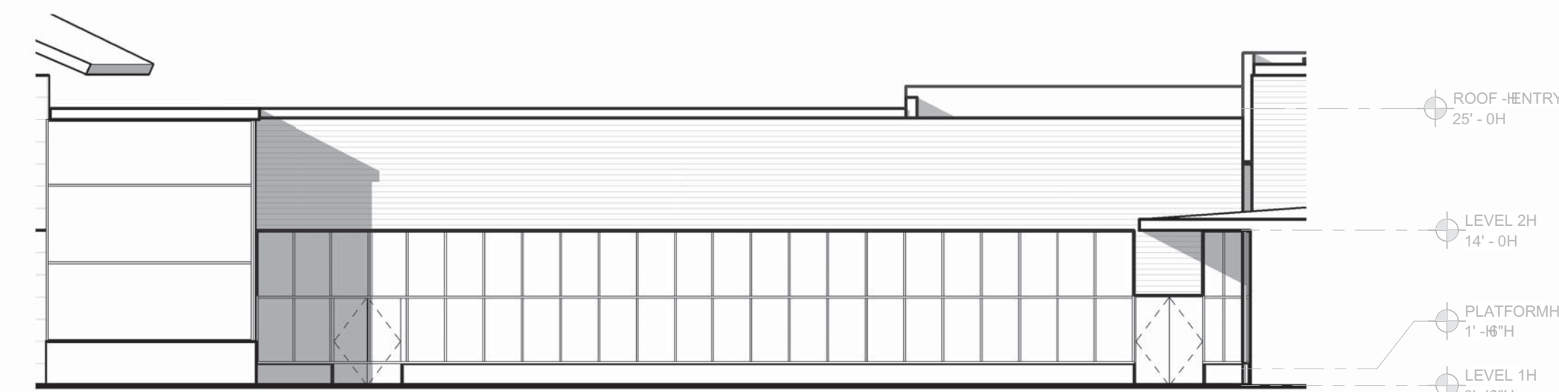
6H EAST ELEVATION - SECTOR BH 3/32" = 1'-0"
