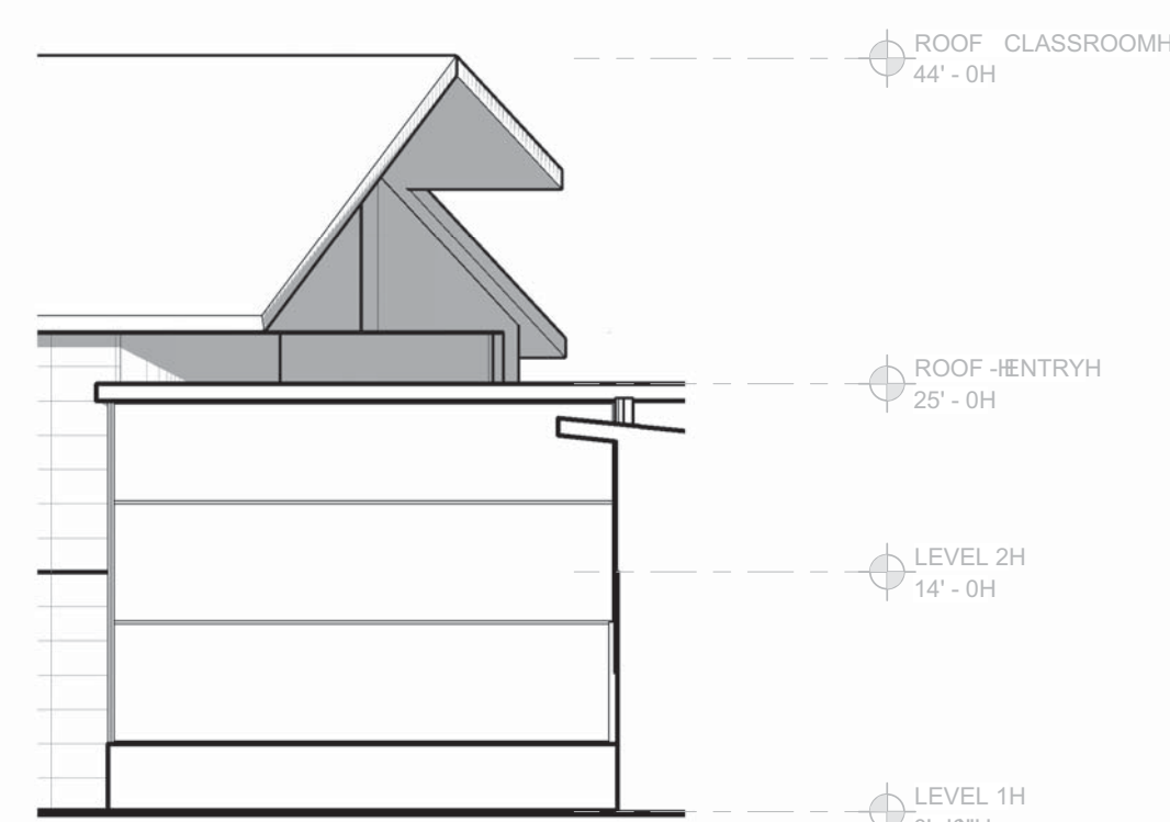
5H NORTH ELEVATION - SECTOR BH 3/32" = 1'-0"
