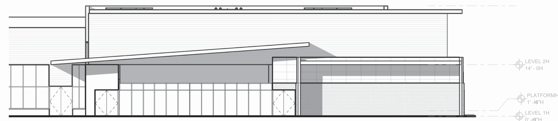
2H EAST ELEVATION - SECTOR AH 3/32" = 1'-0"
