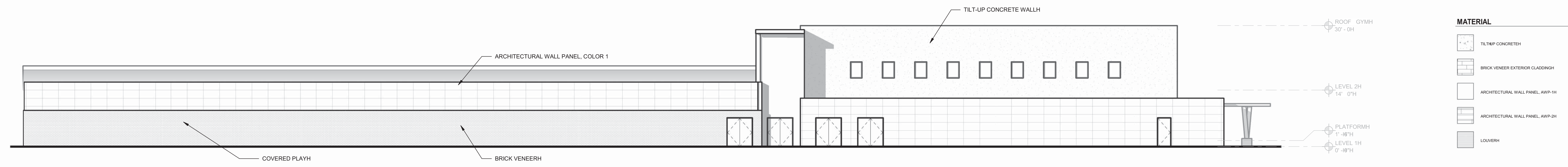
1H NORTH ELEVATION - SECTOR AH 3/32" = 1'-0"
